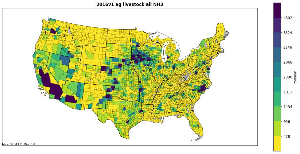
Figure 7. 2016fh ag livestock NH3 emissions by county (tons)
