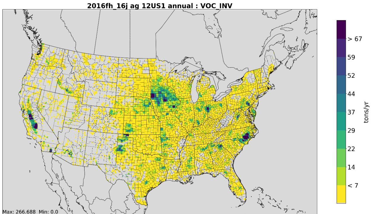
Figure 10. 2016fh ag VOC gridded emissions
