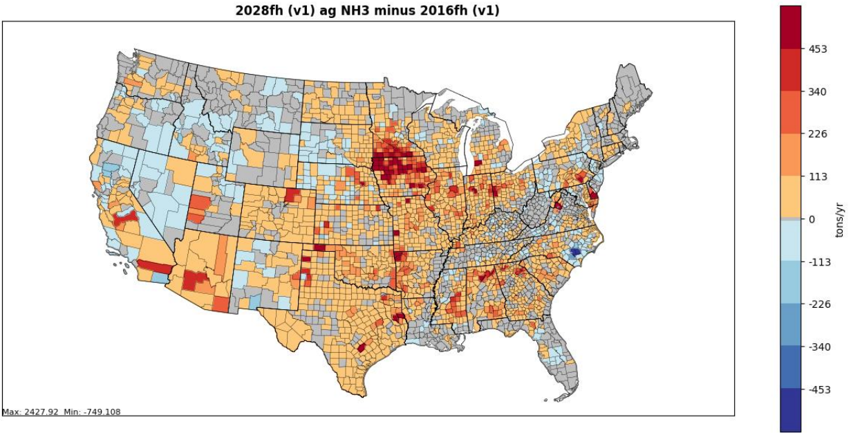
Figure 3. NH3 (tons) Ag Sector Emission Differences between 2028v1 and 2016v1
