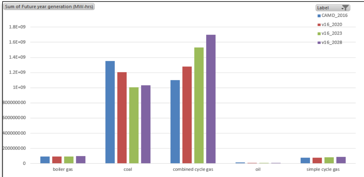
Figure 3: National Generation By Unit Type (MW-Hrs) for Base Year and Future Projections
