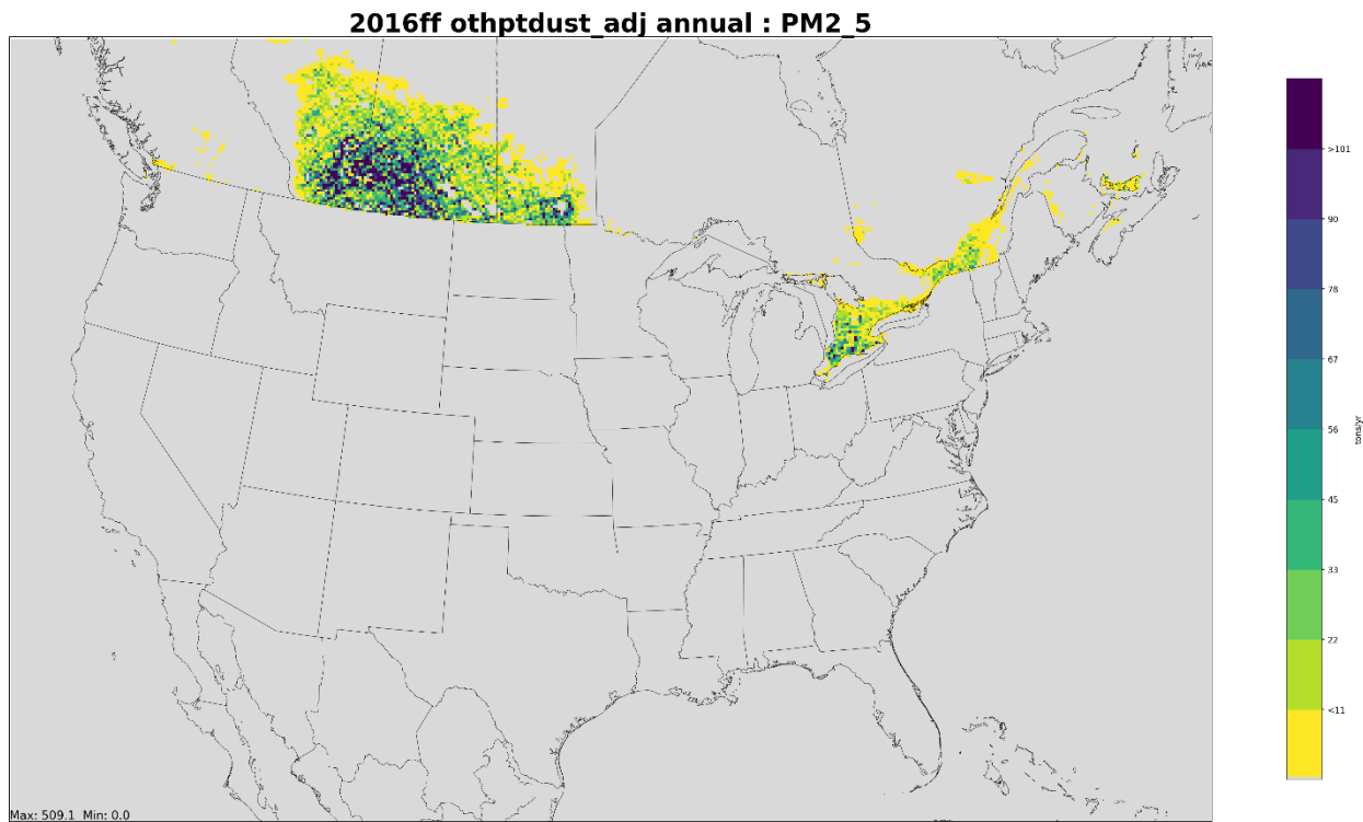
Figure 1. 2016ff 12US1 othptdust annual PM 2.5 emissions with “waffle pattern”
