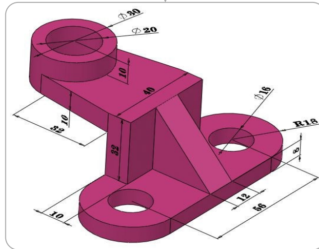
Mechanical Drawings
