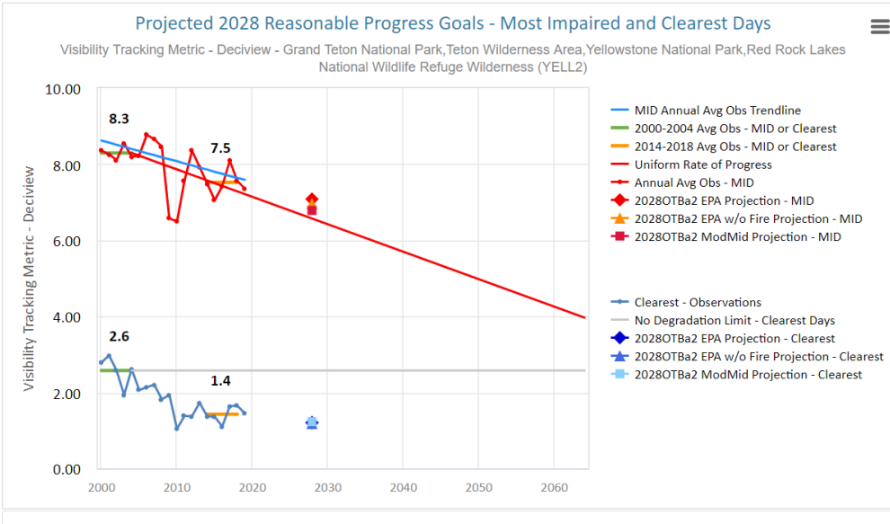
Figure 1. Example URP Glidepath and 2028 visibility projections for Yellowstone National Park, Wyoming from the WRAP TSS Modeling Express Tools Chart 4 (accessed October 21, 2021).
