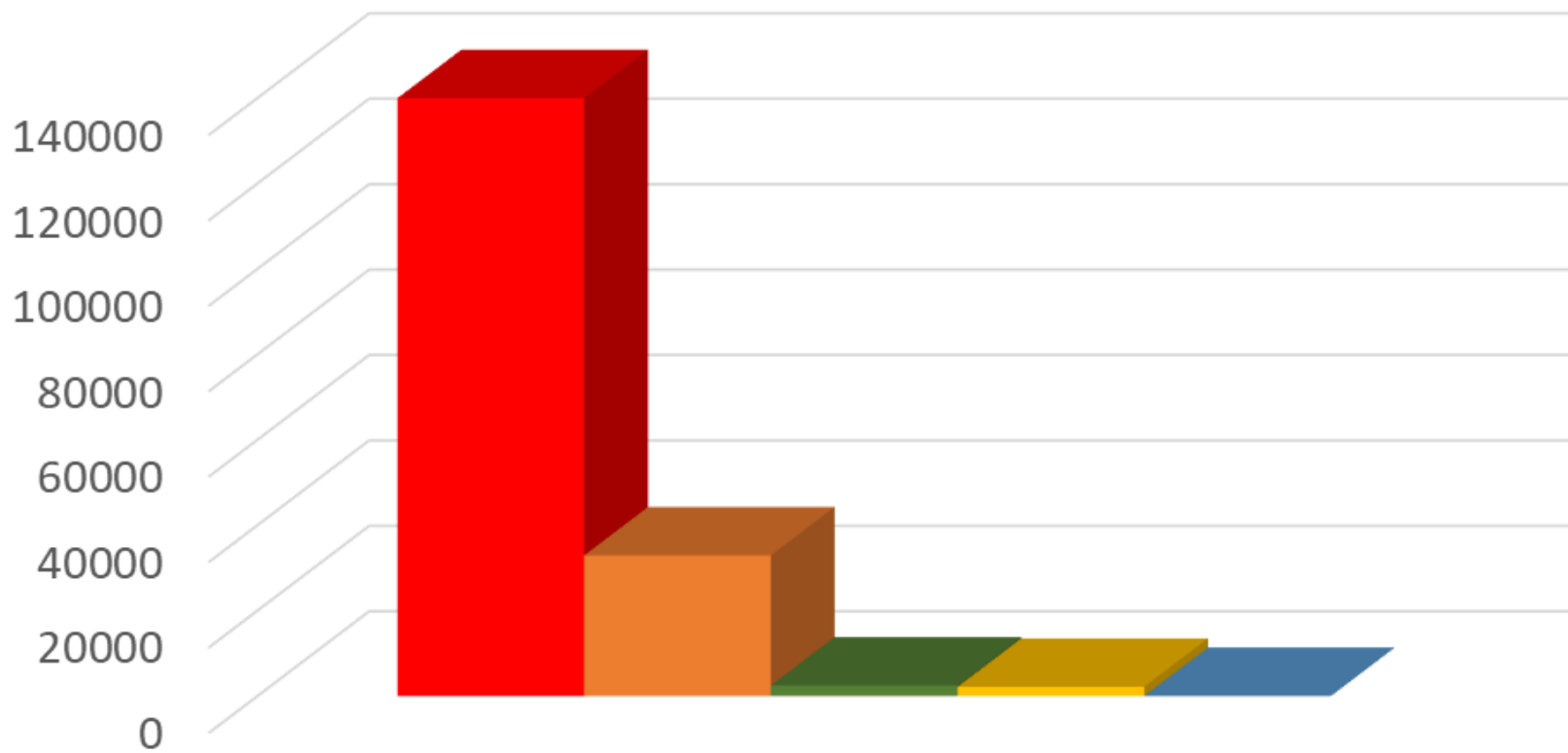
Oil and Gas Point Source: VOC (tons/yr)
