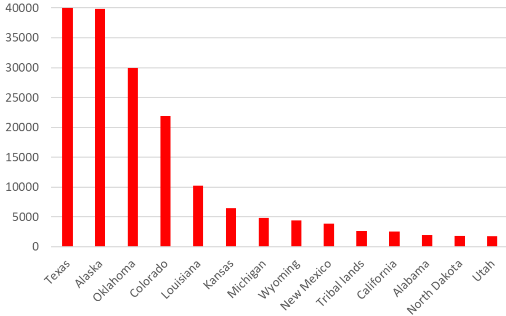
Oil and Gas Point Source: NOx (tons/yr) Gathering/Processing/Production
