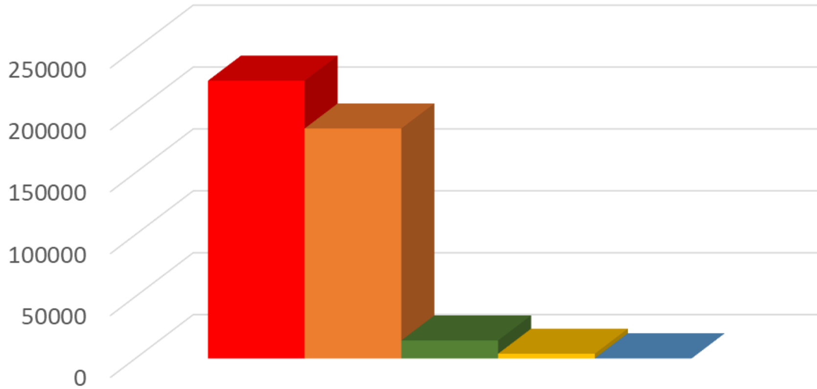
Oil and Gas Point Source: NOx (tons/yr)
