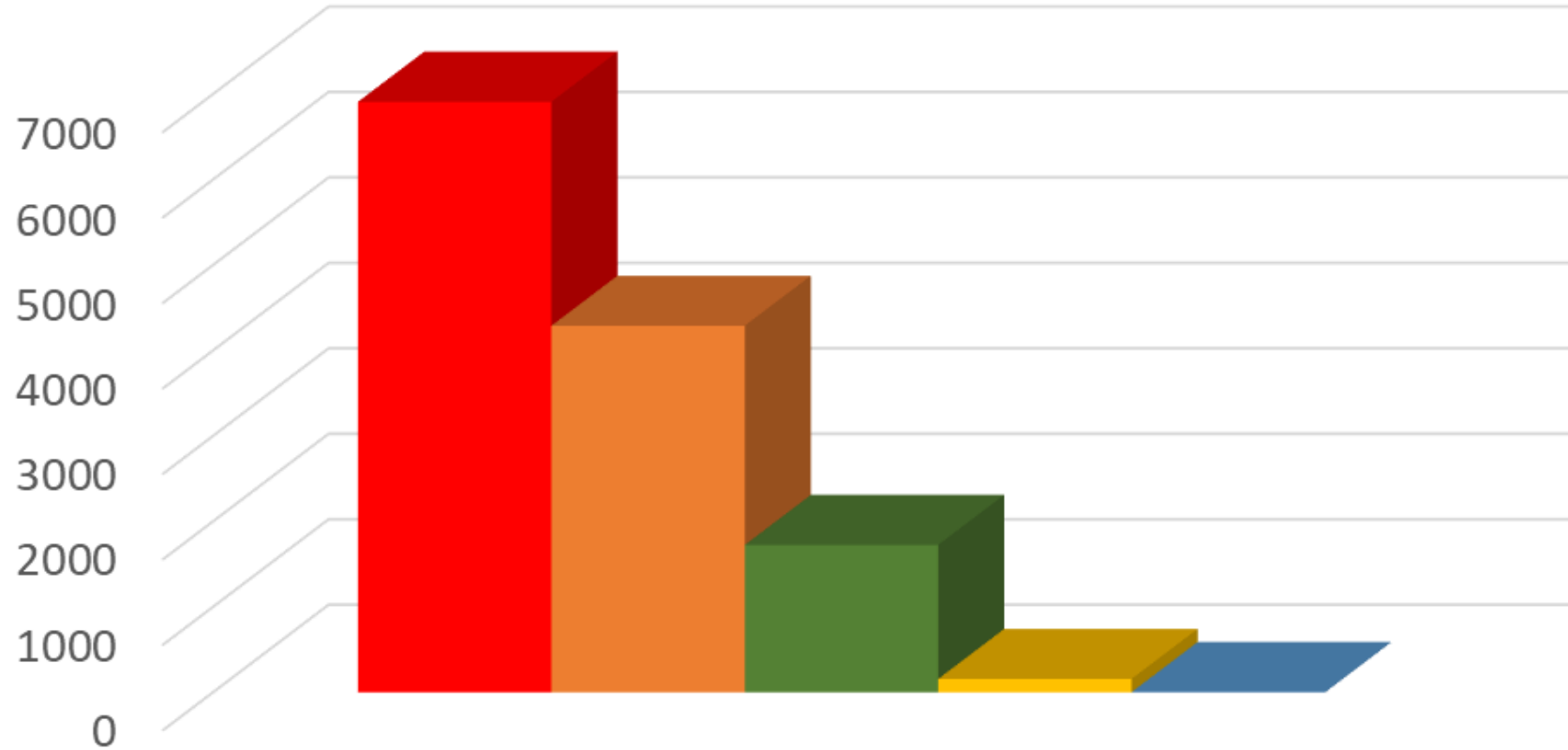
Oil and Gas Point Source: PM2_5 (tons/yr)
