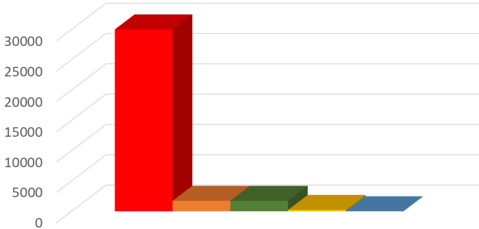
Oil and Gas Point Source: SO2 (tons/yr)
