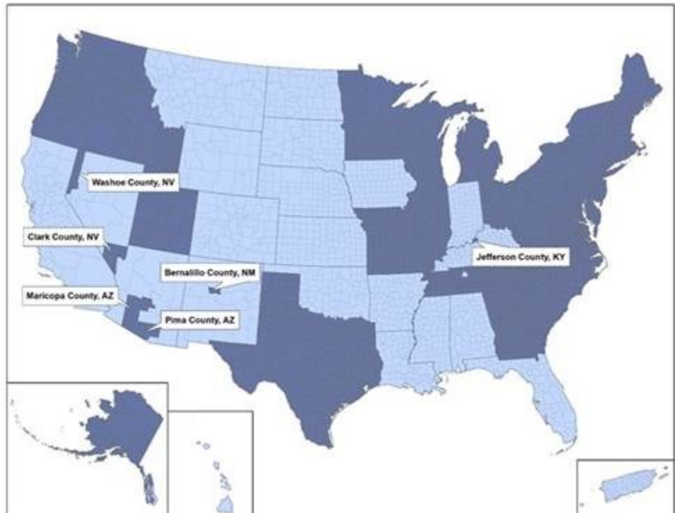
Map image above shows ID, OR, and WA and Maricopa and Pima Counties in AZ, Clark and Washoe Counties in NV, and Bernalillo County in NM submitted activity data for MOVES to populate the 2014 NEI. CA submits mobile source emissions directly (output from EMF).
